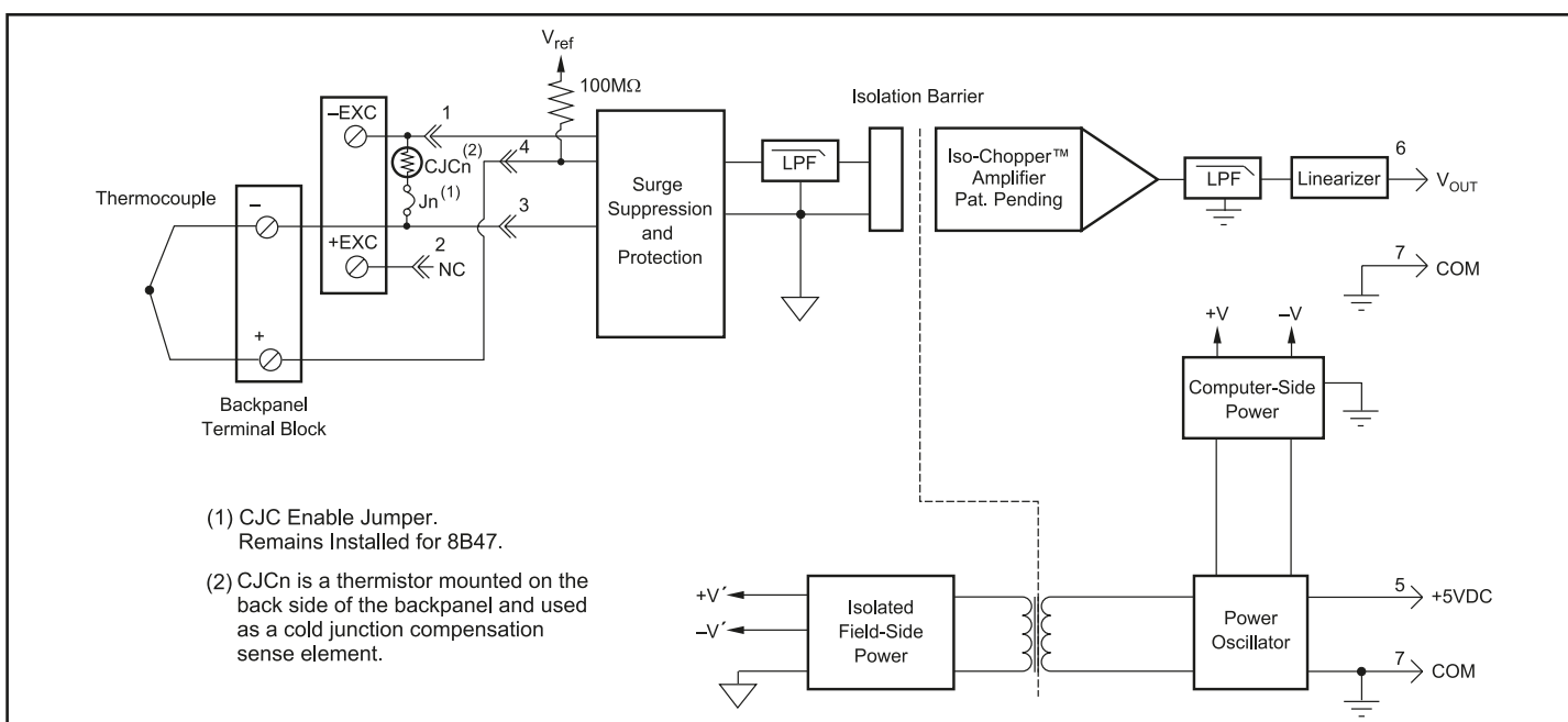
Figure 1: 8B47 Block Diagram
