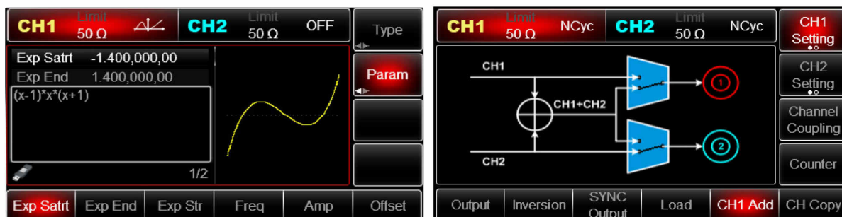
Built-in 16 harmonic generator
