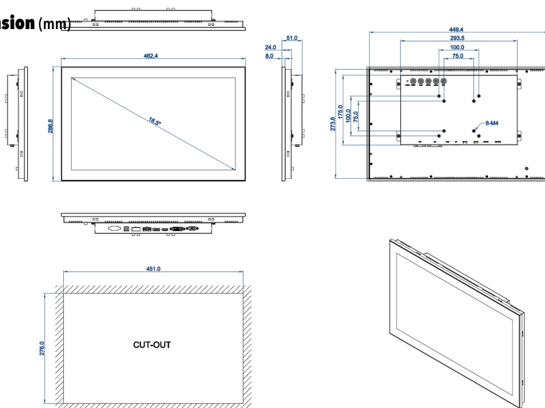
DIMENSIONAL DRAWING:TM-PCA185
