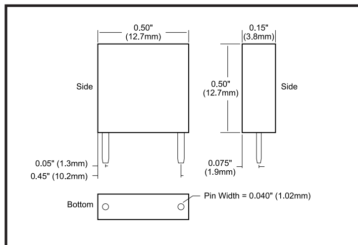
Figure 23: SCMXR1 Physical Dimensions
