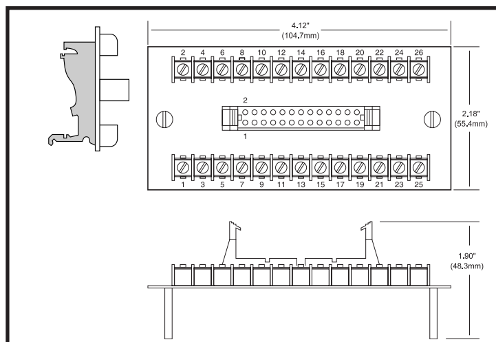
Figure 20: SCMXIF Universal Interface Board Dimensions
