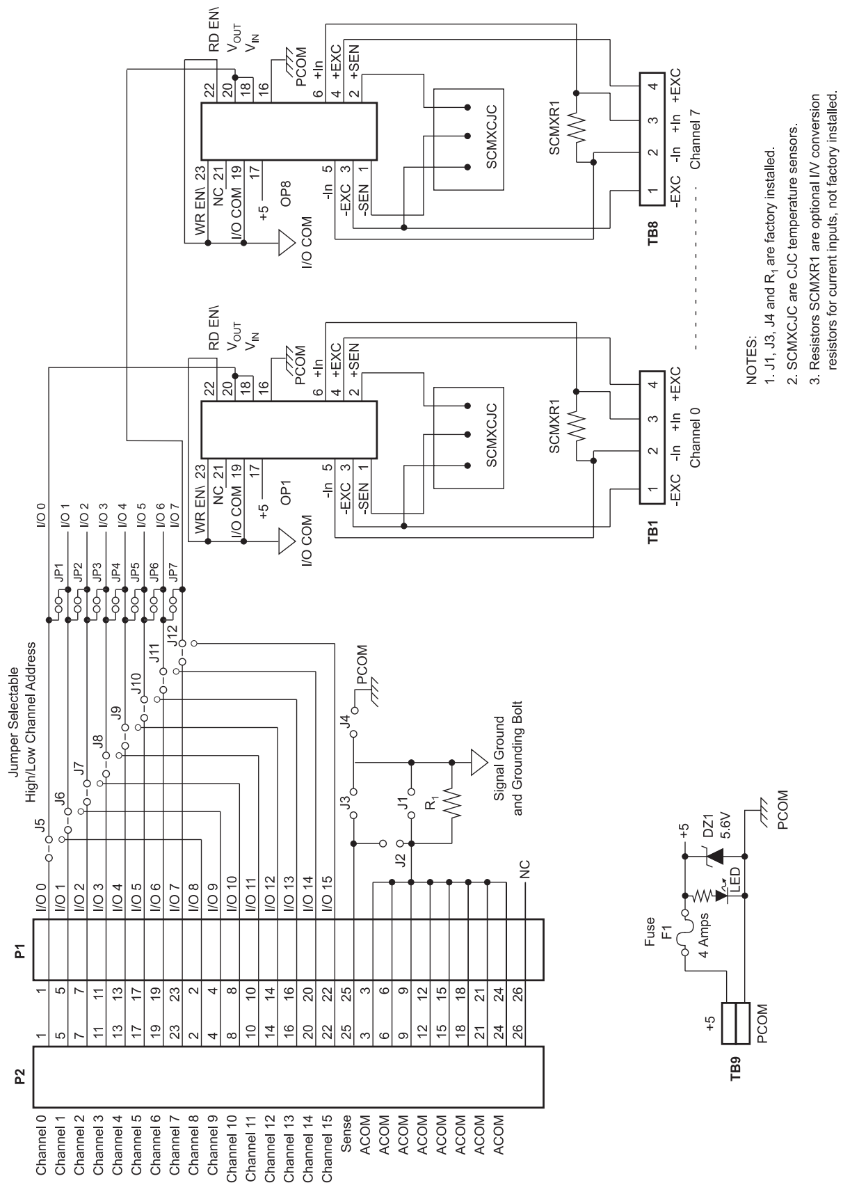
Figure 13: SCMPB05 Schematic
