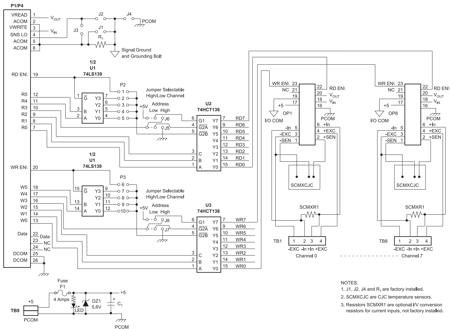
Figure 15: SCMPB06 Schematic
