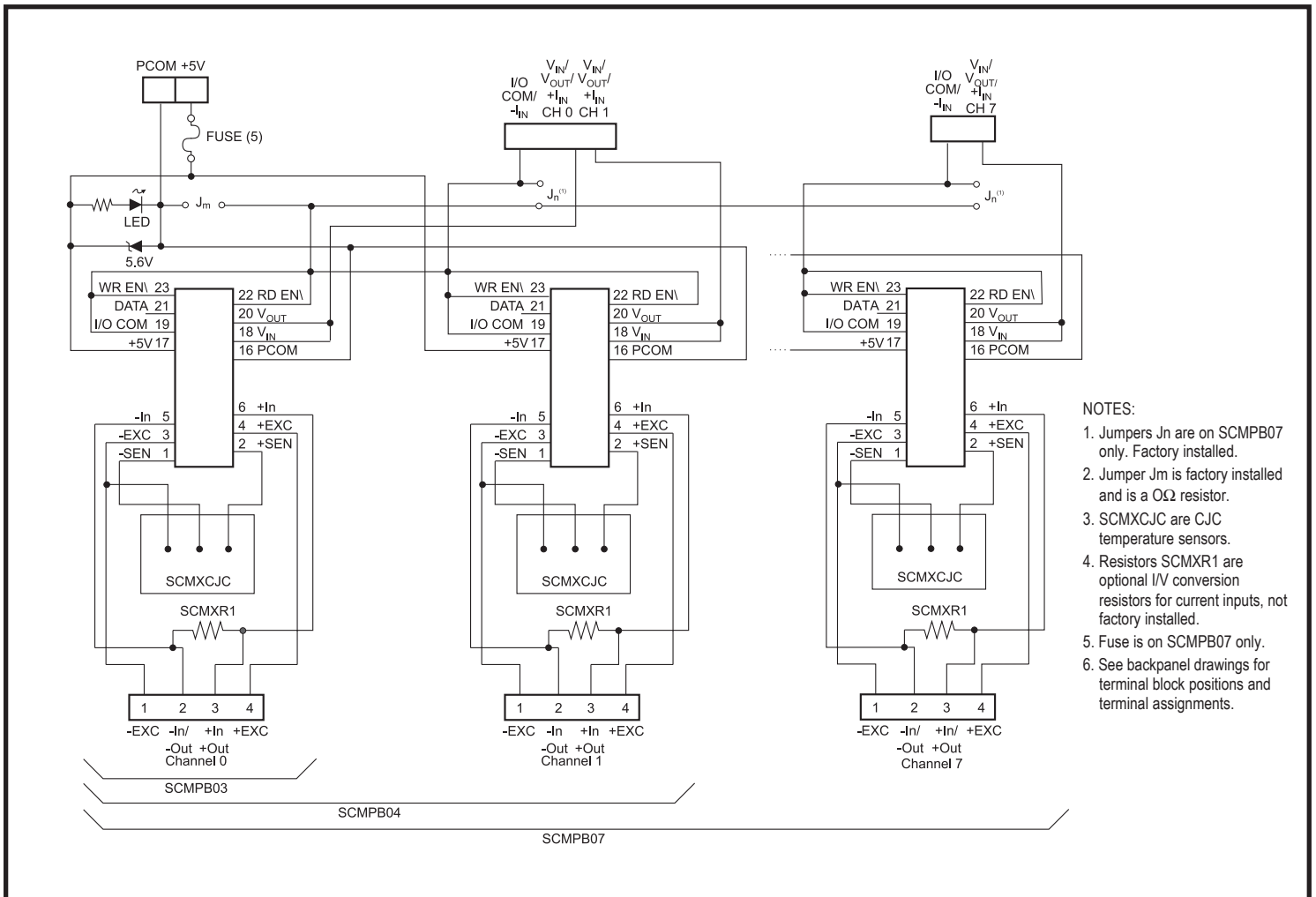
Figure 11: SCMPB03/SCMPB04/SCMPB07 Schematic
