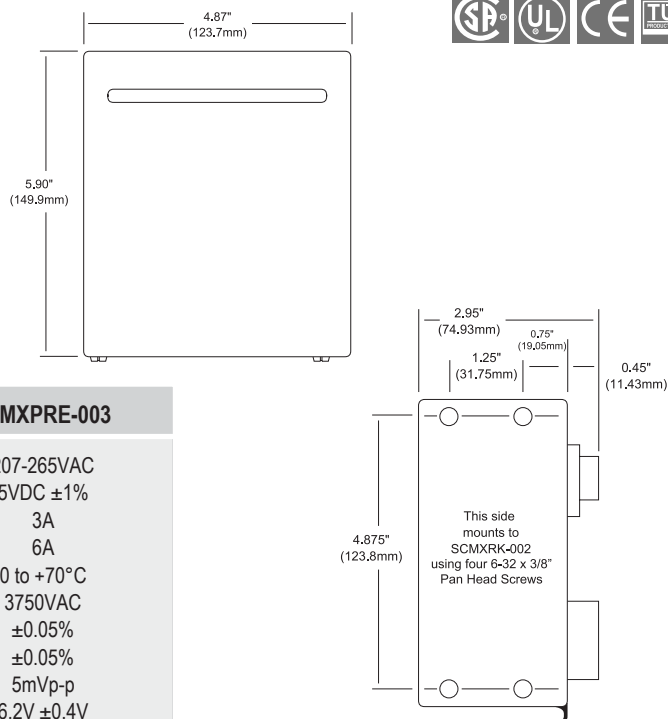
Figure 26: SCMXPRT-003/SCMXPRE-003 Physical Dimensions
