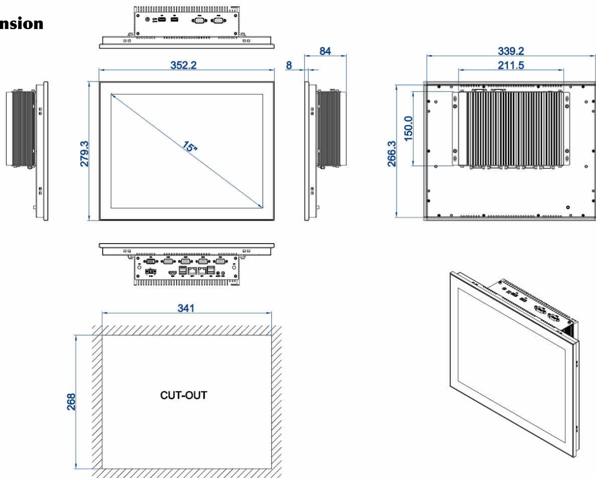
DIMENSIONAL DRAWING:TPC-PC150
