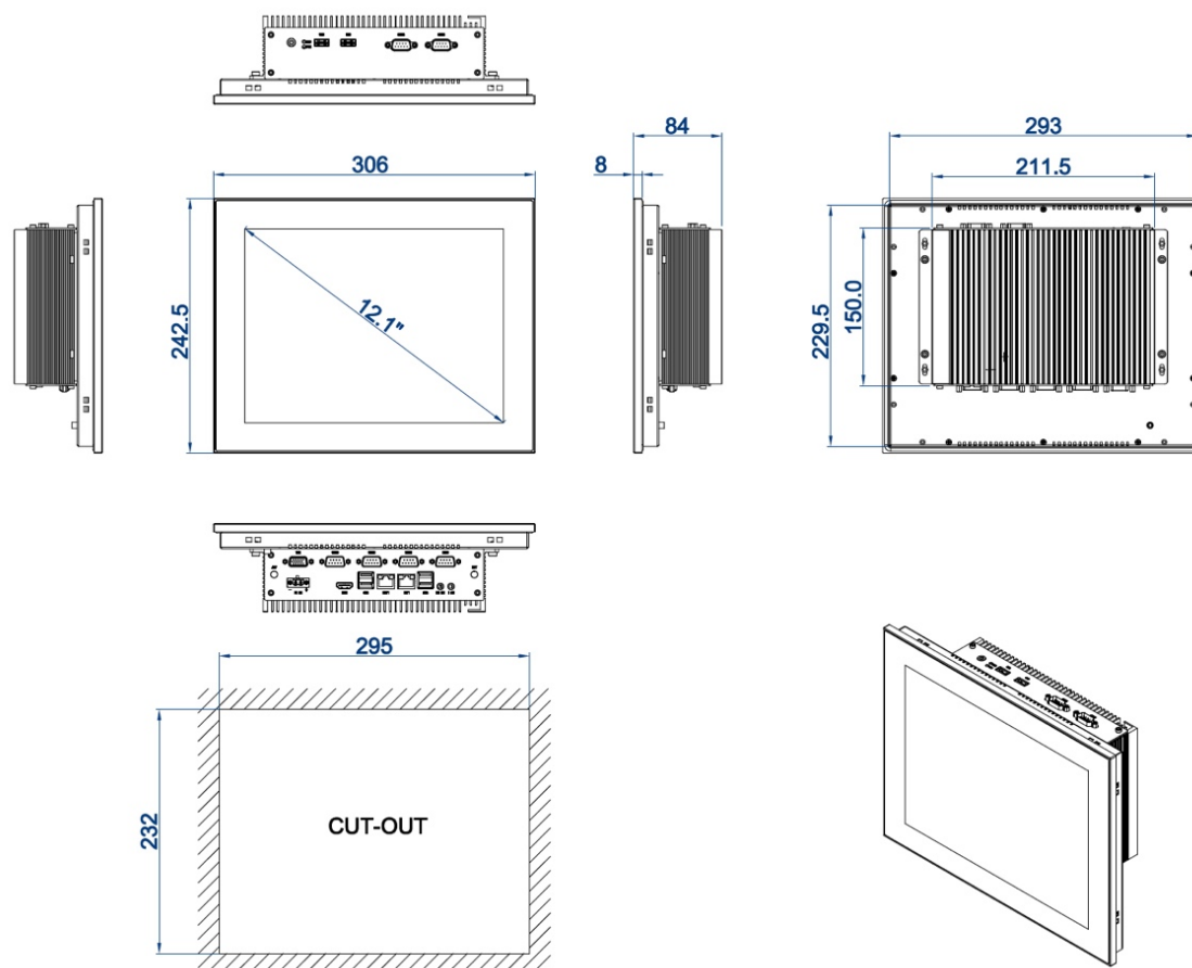
DIMENSIONAL DRAWING:TPC-PC121
