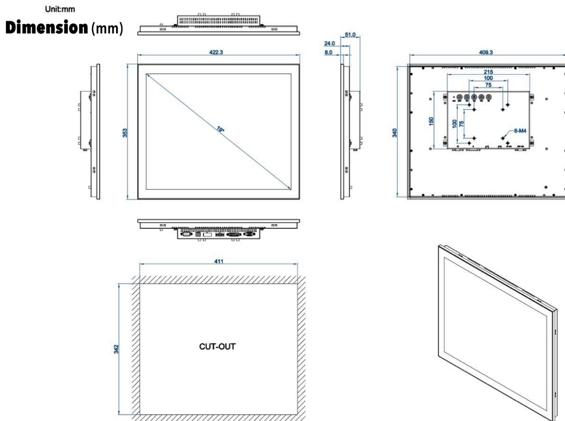
DIMENSIONAL DRAWING:TM-PC190
