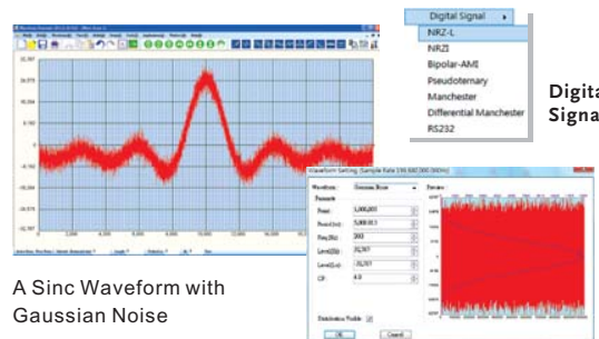
Gaussian Noise
