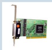
UC-756 uPCI 4xRS232 DB25
