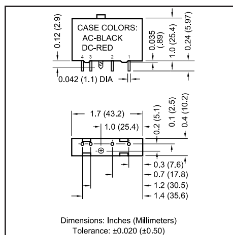
Figure 1: SCMD-MOAC/MODC Physical Dimensions
