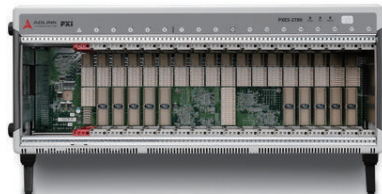
PXES-2780 Hybrid Peripheral Slots
