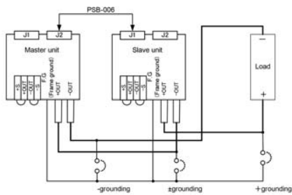
Series Connection
