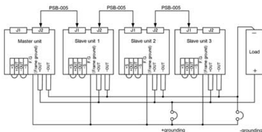
Parallel Connection
